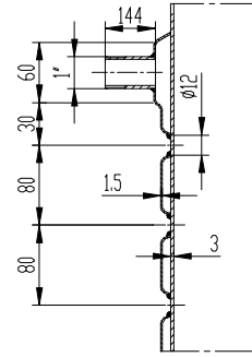
cooling jacket
